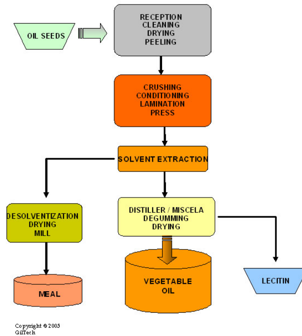
Figure 13 VEGETABLE OILS - FLUXOGRAM
