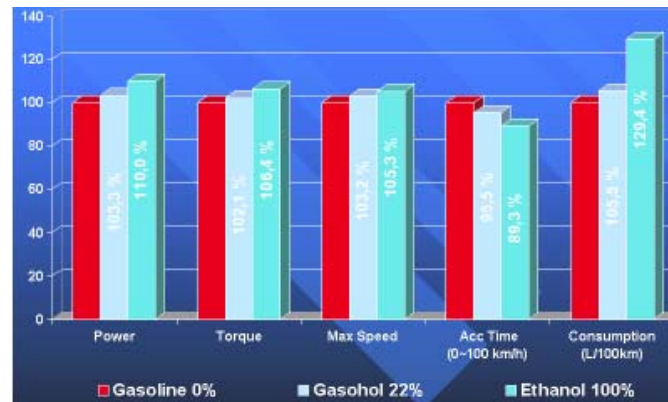
Figure 5 – Relative performance of ethanol engines [6]
